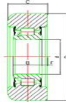
Forklift Mast Roller (MG**R1-*)
