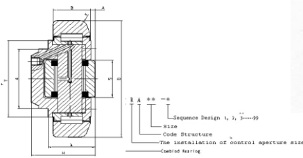
Standard combination bearings (CRA**.**)
