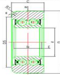
Forklift Mast Roller (MG**B7-*)
