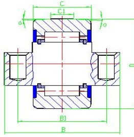
forklift side roller (SR**NR***)
