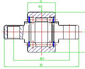
forklift side roller (SR**D***)
